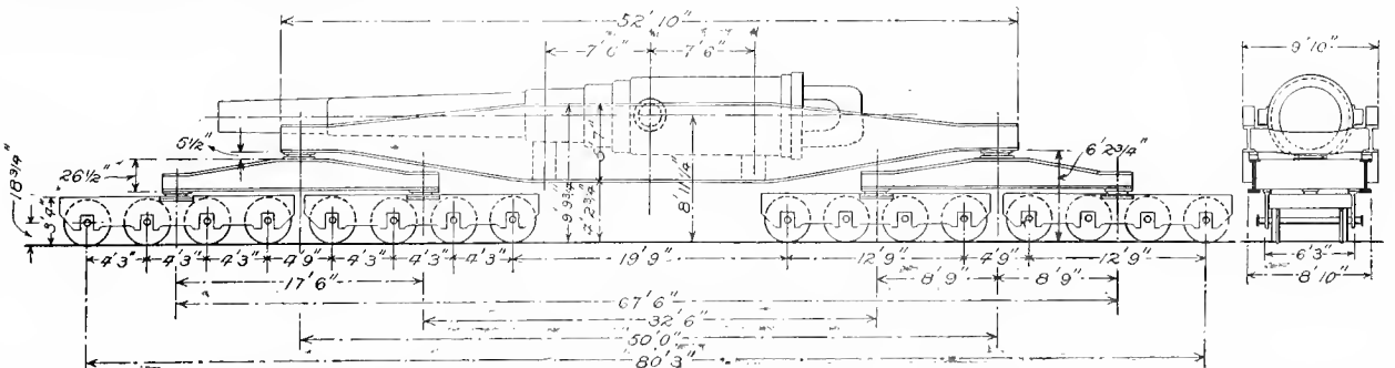
Figs. 4804-4805. SPECIAL TRUCK FOR CONVEYING LARGE GUNS. PENNSYLVANIA RAILROAD COMPANY.
